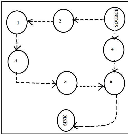
Fig1: An overview of fig specifying stretch attack
