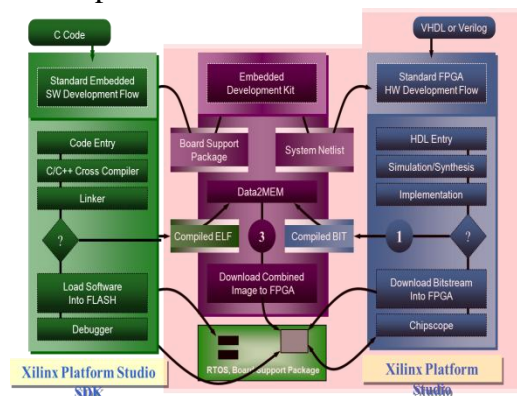
Fig 1: Embedded Development Kit Design Flow
